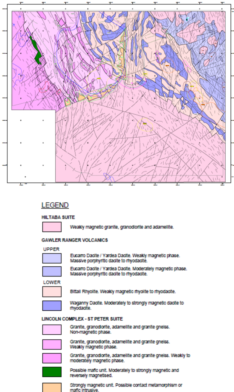
Figure 4: Geological interpretation of tenement area derived from the aeromagnetic image comprising Figure 3. The southern sector is interpreted as part of a large Hiltaba Suite granite pluton while the north eastern sector comprises about 70% exposed and interpreted Gawler Range Volcanics (GRV). The north eastern and north western sectors are separated by a north-trending imbricate zone, also interpreted as GRV. The north western sector is interpreted to comprise about 25% GRV in the east abutting, to the west, about 75% Lincoln Complex – St Peter Suite dominantly composed of variable, but weakly magnetized granitic rocks and granite gneiss. The north western sector is partly bordered by a fringe of magnetized material against the north eastern and southern sectors. This fringe is interpreted as a contact metamorphic effect.
