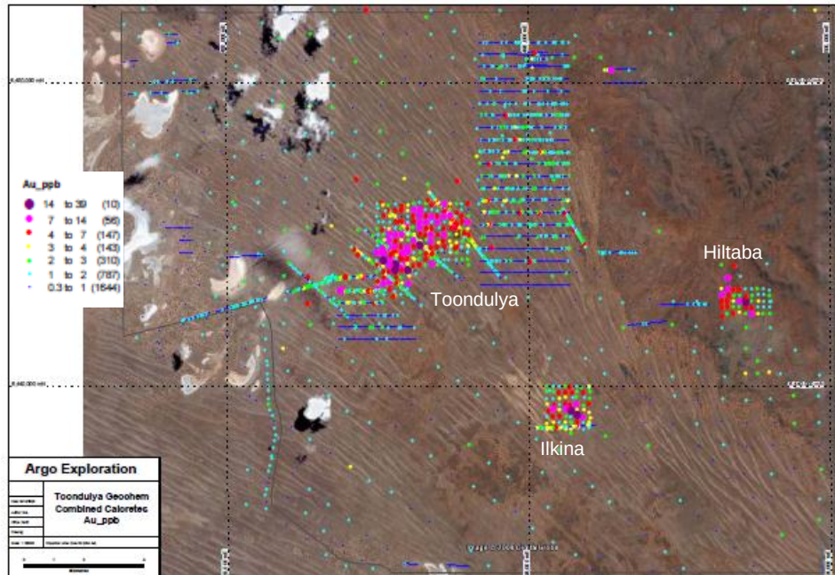
Figure 1: EL4284 showing calcrete sample locations and associated gold values superimposed upon satellite imagery of the area. The image illustrates the distribution of the mantling, north west-trending sand dune field, with minor associated saline clay pans and ephemeral lakes. Exposures of Hiltaba Suite granite and Gawler Range Volcanics are evident in the north eastern corner of the tenement.
