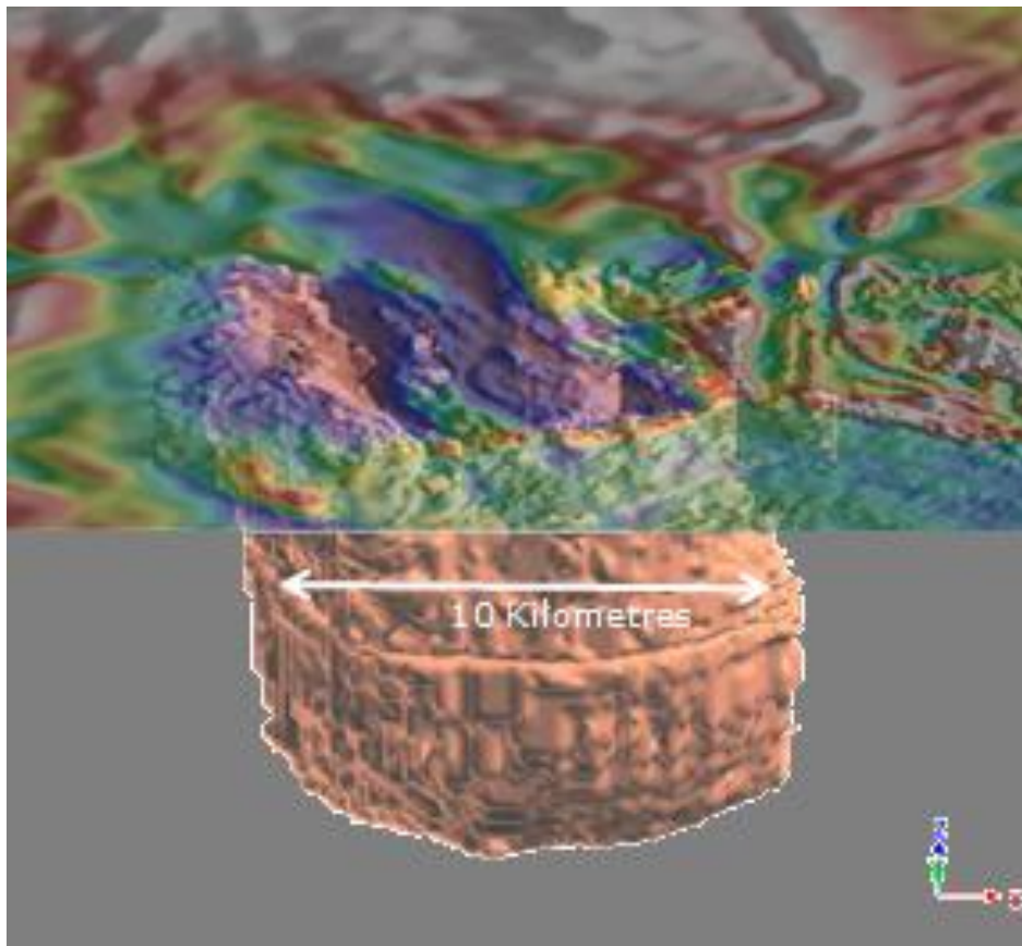
Figure 10: Reduced to Pole Total Magnetic Intensity image draped over 3-D model of pluton, looking north. Note that the overall pluton is generally coincident with an extensive magnetic low and that specific apophyses also coincide with magnetic lows. Note also the close approach to surface of apical projections of the apophyses.
